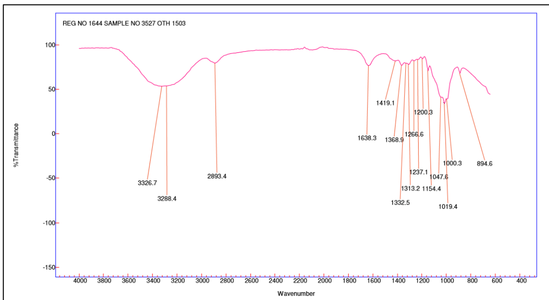
Graph 1: FTIR graph of the Bambo-OFF (Offshoot 100% BAMBOO WET WIPES)
