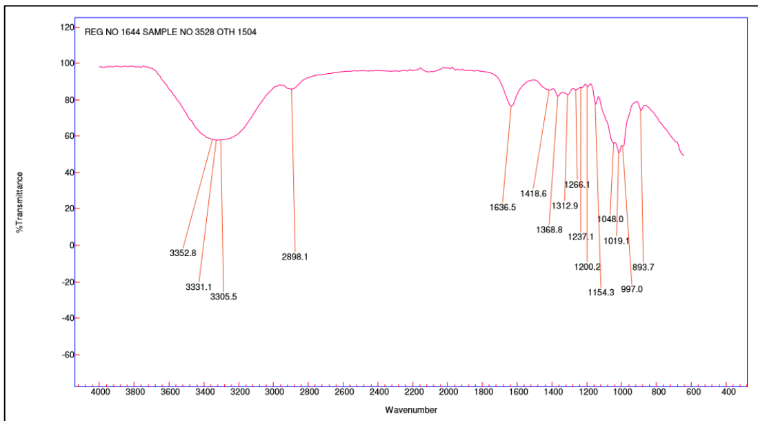
Graph 1: FTIR graph of the Viscose-OFF (Offshoot 100% VISCOSE WET WIPES)
