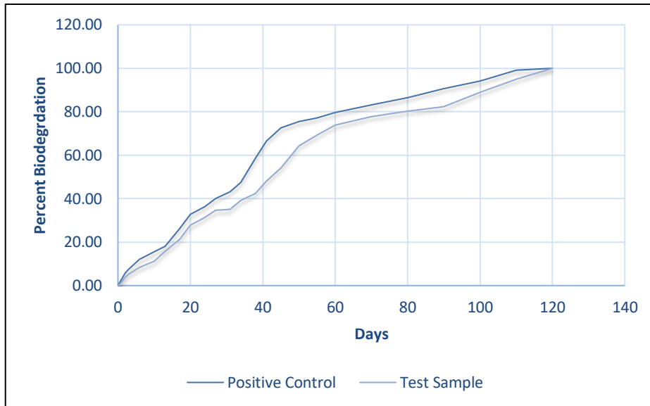
Graph 2: Percentage biodegradation of Viscose-OFF (Offshoot 100% VISCOSE WET WIPES) Sample under aerobic composting
